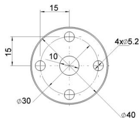
Propeller Drilling
