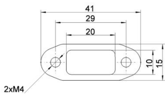
Muffler Interface
